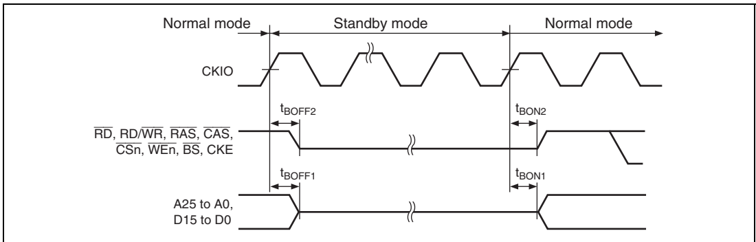
Figure 21.9 Pin Drive Timing in Standby Mode
