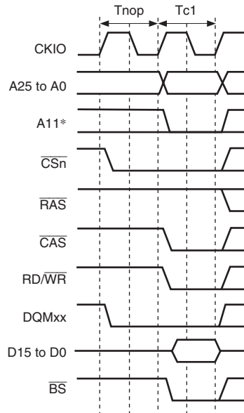
Figure 7.21 Single Write Timing (Bank Active, Same Row Address)
